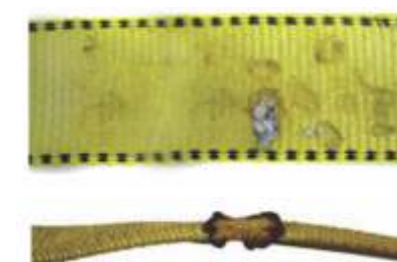
Sling Weld Splatters and Charring/Melting
